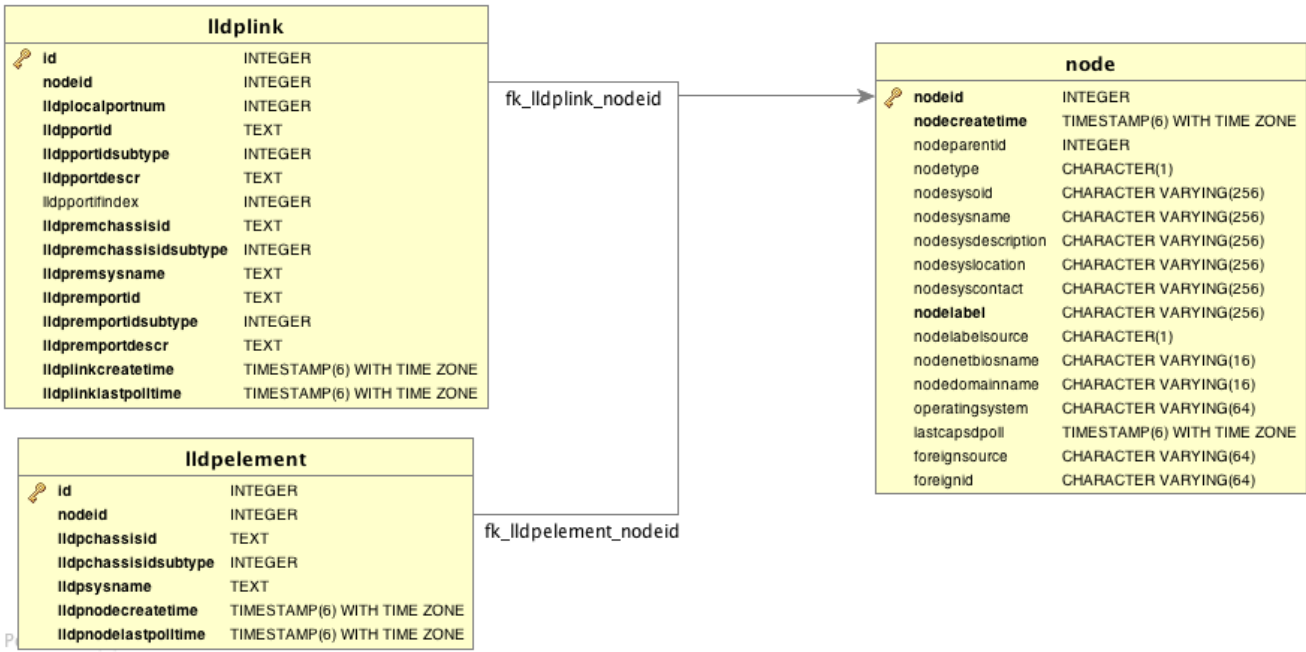
Figure 40. Database tables related to LLDP discovery
