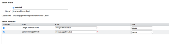
Figure 8. Configure MBean attributes for data collection configuration
