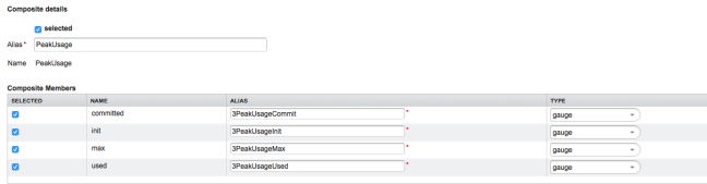
Figure 9. Configure Composite attributes for data collection configuration
